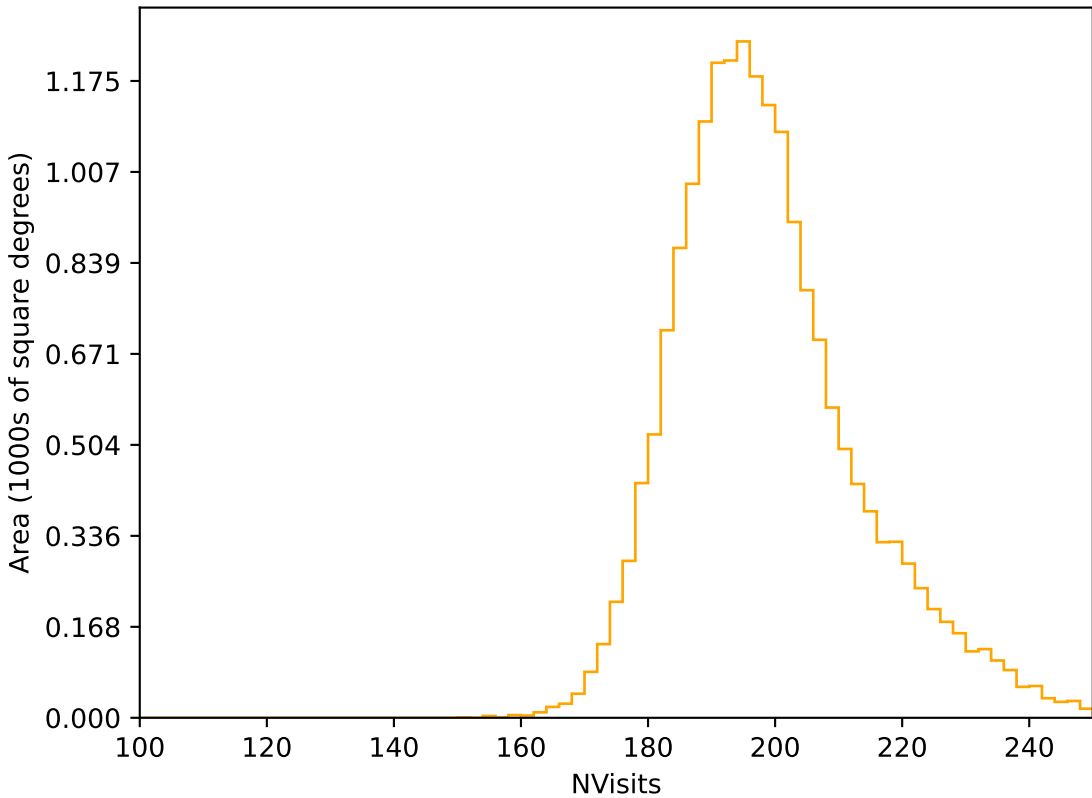
weather_cloudso12v3.4_10yrs WFD r band: NVisits
