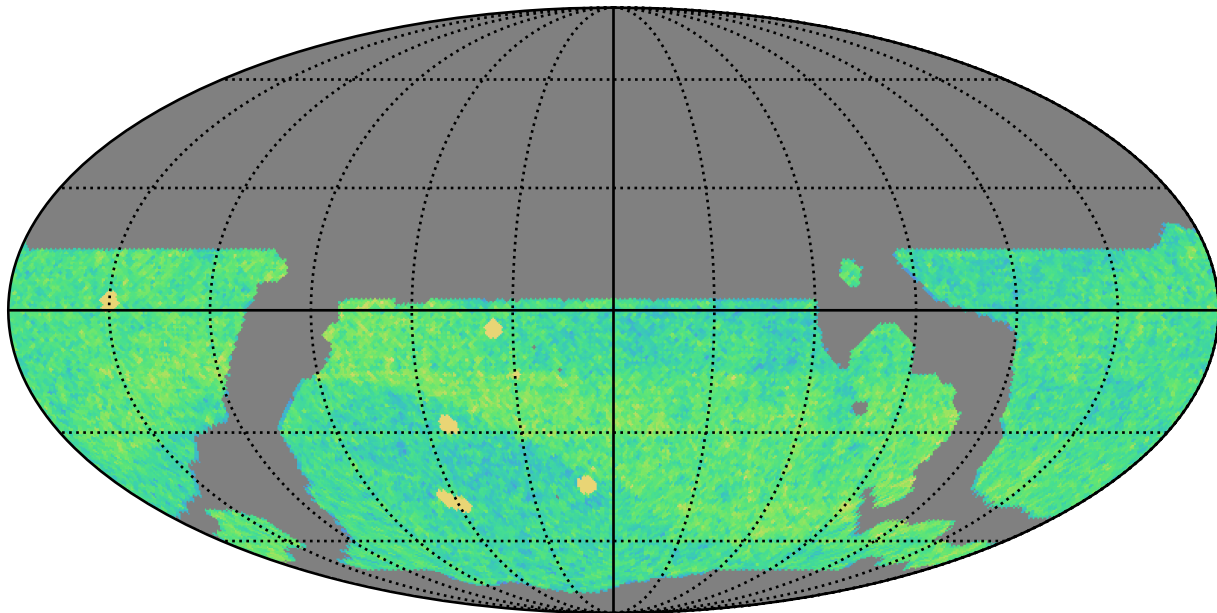
weather_cloudso12v3.4_10yrs WFD i band: NVisits
