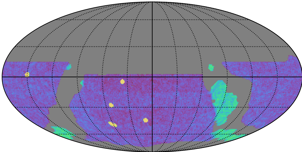
weather_cloudso12v3.4_10yrs WFD g band: NVisits
