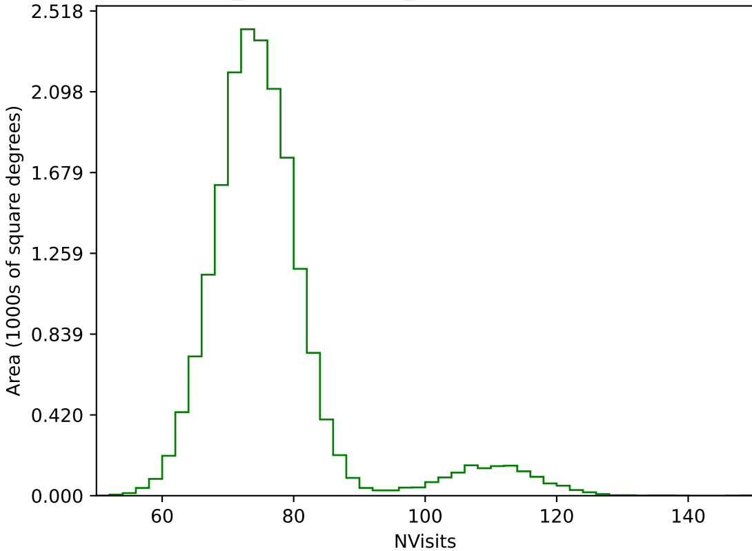
weather_cloudso12v3.4_10yrs WFD g band: NVisits
