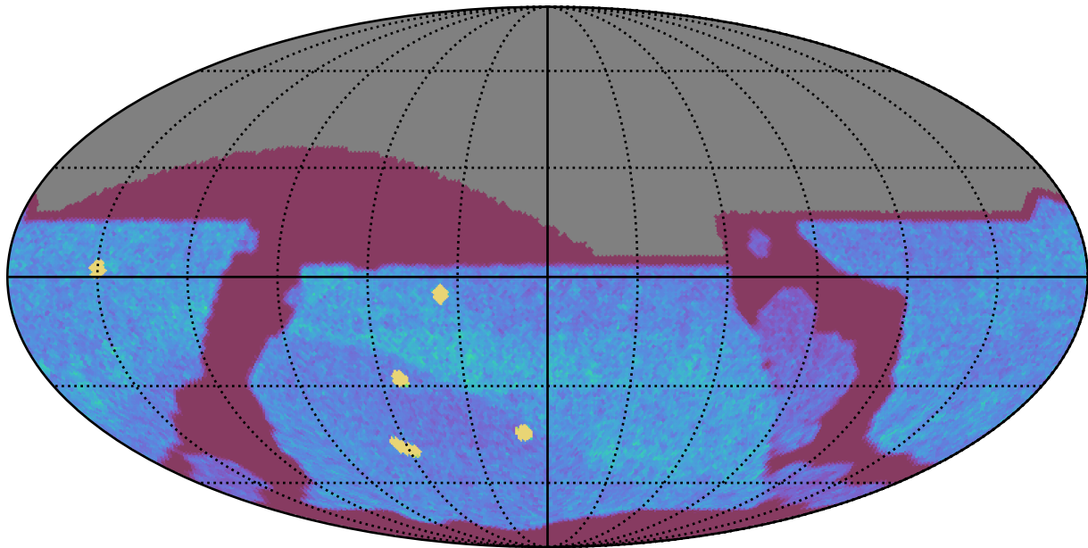
weather_cloudso12v3.4_10yrs All sky z band: NVisits
