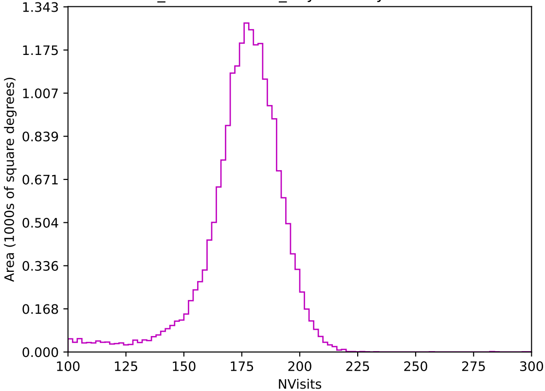
weather_cloudso12v3.4_10yrs All sky z band: NVisits
