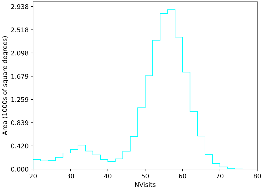
weather_cloudso12v3.4_10yrs All sky u band: NVisits
