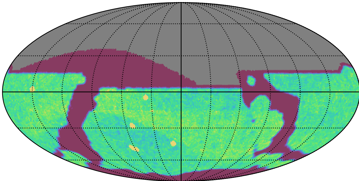
weather_cloudso12v3.4_10yrs All sky i band: NVisits
