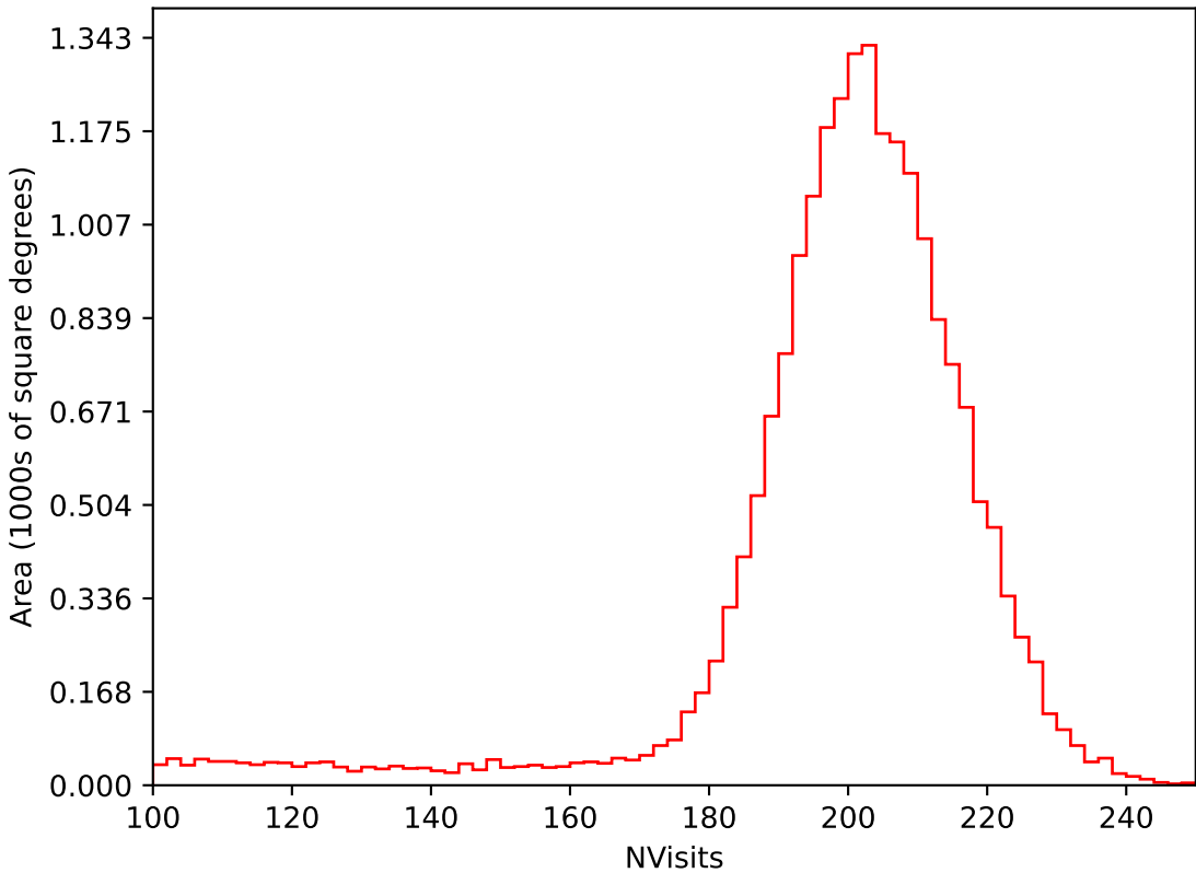
weather_cloudso12v3.4_10yrs All sky i band: NVisits
