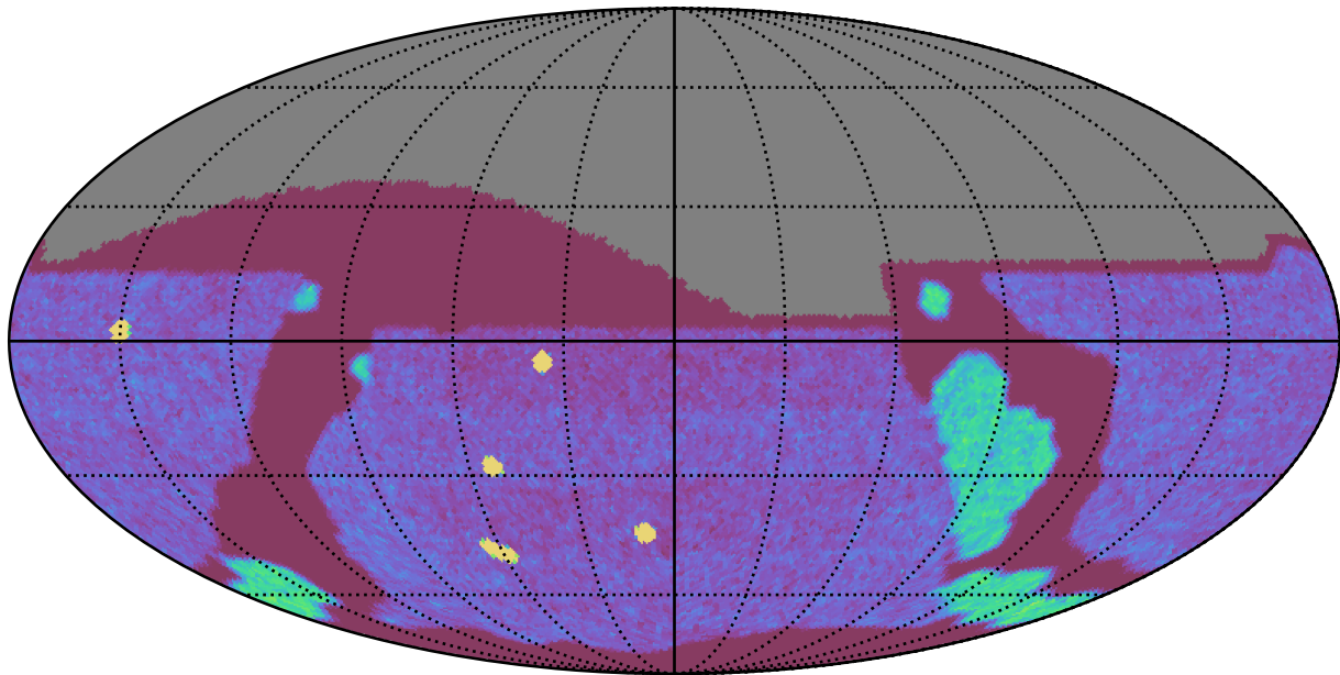
weather_cloudso12v3.4_10yrs All sky g band: NVisits
