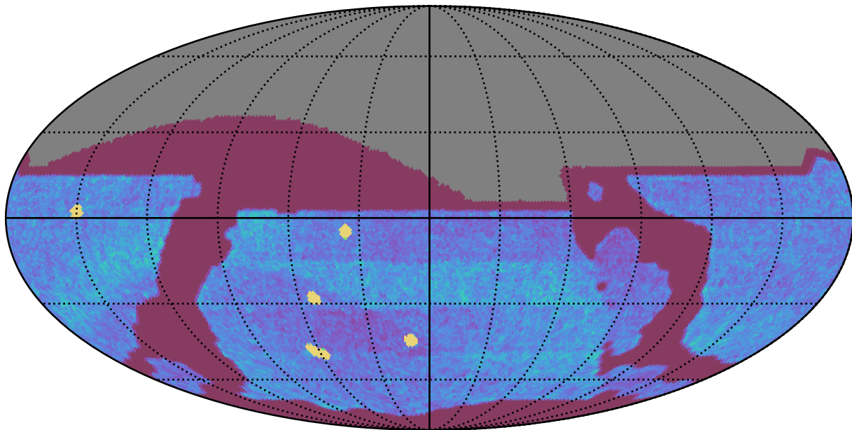
weather_cloudso12v3.4_10yrs All sky all bands: NVisits
