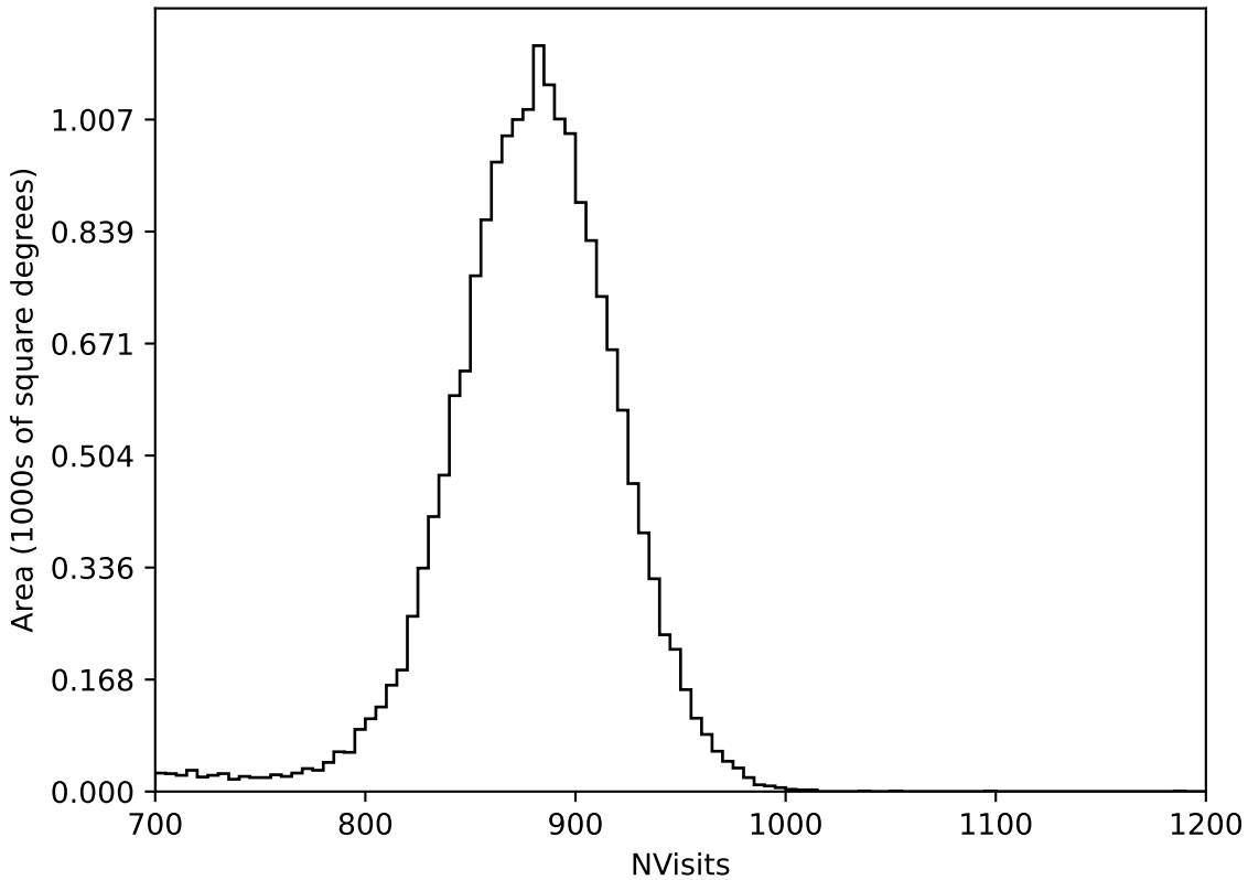
weather_cloudso12v3.4_10yrs All sky all bands: NVisits
