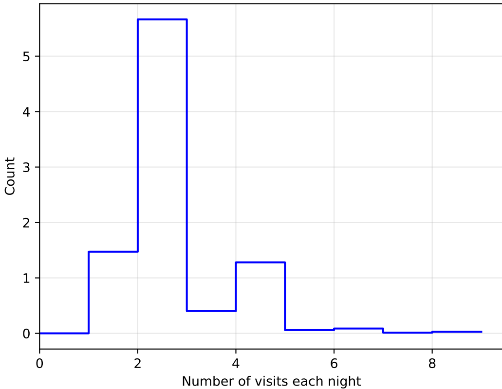
1e6 weather_cloudso12v3.4_10yrs WFD: NVisitsPerNight
