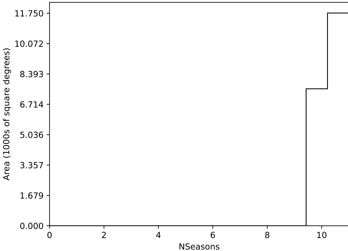
weather_cloudso12v3.4_10yrs WFD all bands: NSeasons
