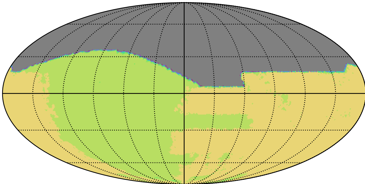
weather_cloudso12v3.4_10yrs All sky all bands: NSeasons
