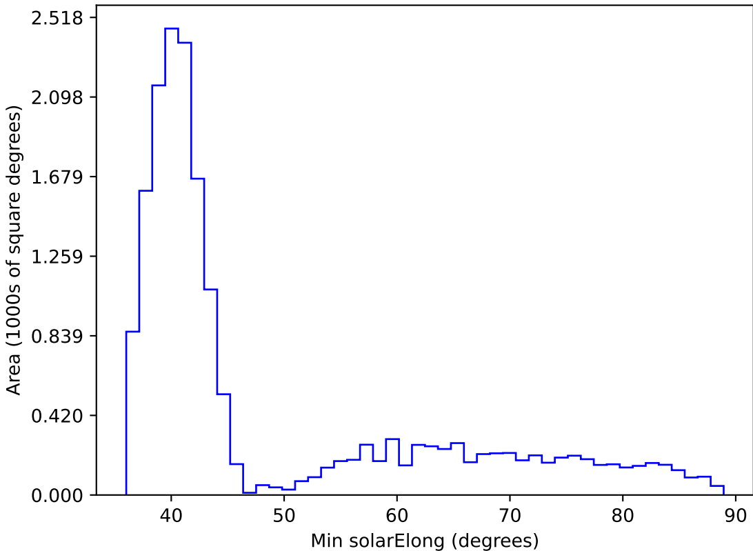
weather_cloudso12v3.4_10yrs WFD z band: Min solarElong
