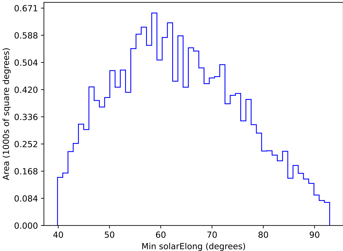
weather_cloudso12v3.4_10yrs WFD y band: Min solarElong
