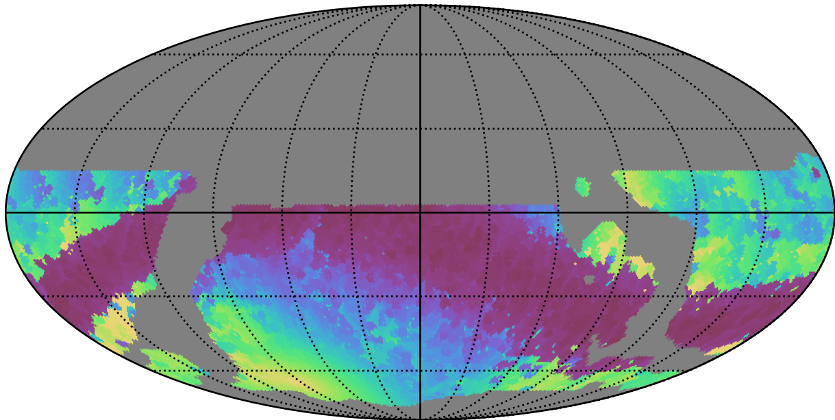
weather_cloudso12v3.4_10yrs WFD r band: Min solarElong
