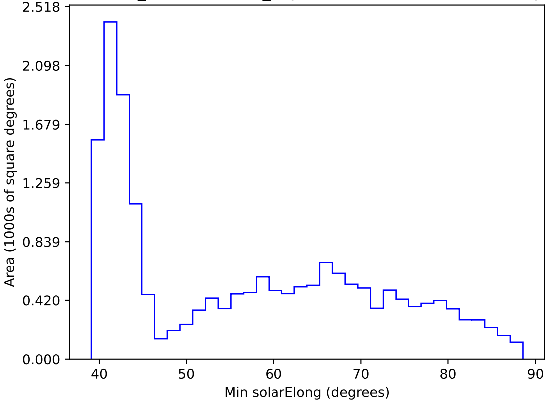
weather_cloudso12v3.4_10yrs WFD r band: Min solarElong
