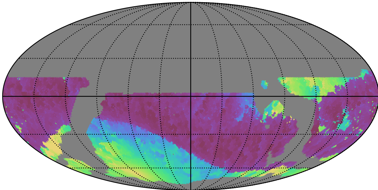
weather_cloudso12v3.4_10yrs WFD i band: Min solarElong
