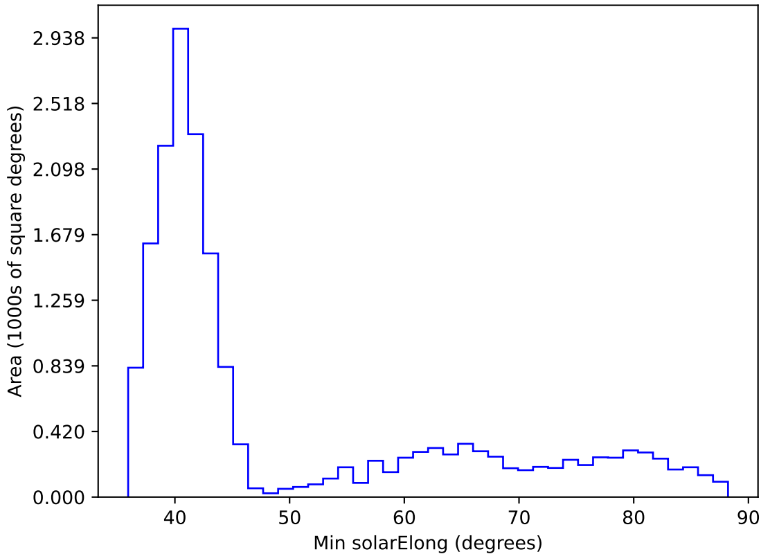
weather_cloudso12v3.4_10yrs WFD i band: Min solarElong
