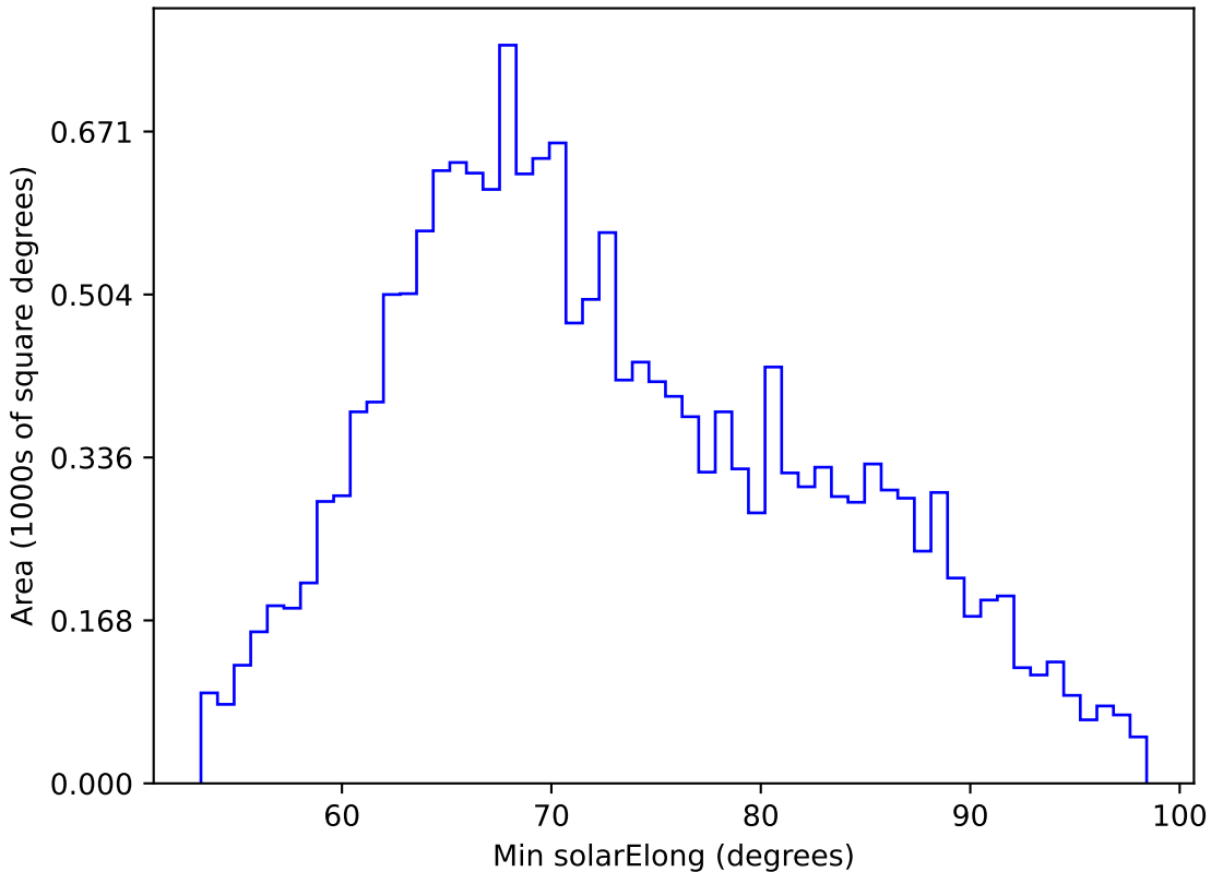
weather_cloudso12v3.4_10yrs WFD g band: Min solarElong
