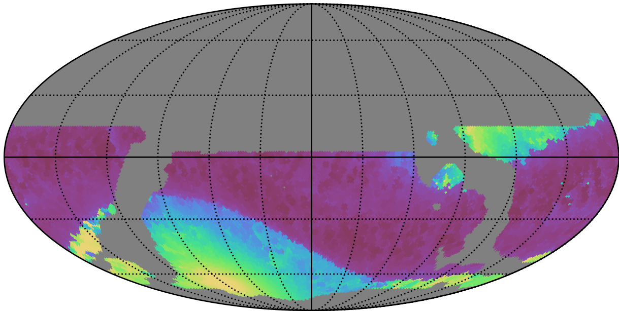
weather_cloudso12v3.4_10yrs WFD all bands: Min solarElong
