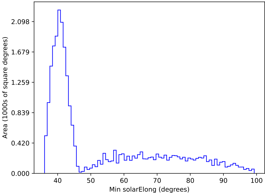
weather_cloudso12v3.4_10yrs All sky z band: Min solarElong
