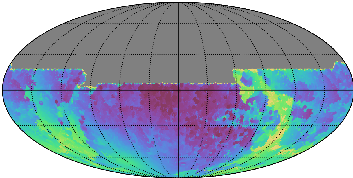
weather_cloudso12v3.4_10yrs All sky y band: Min solarElong
