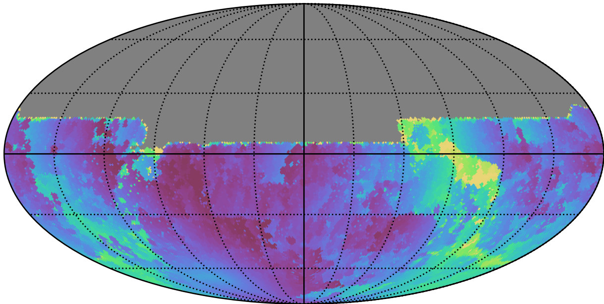
weather_cloudso12v3.4_10yrs All sky u band: Min solarElong
