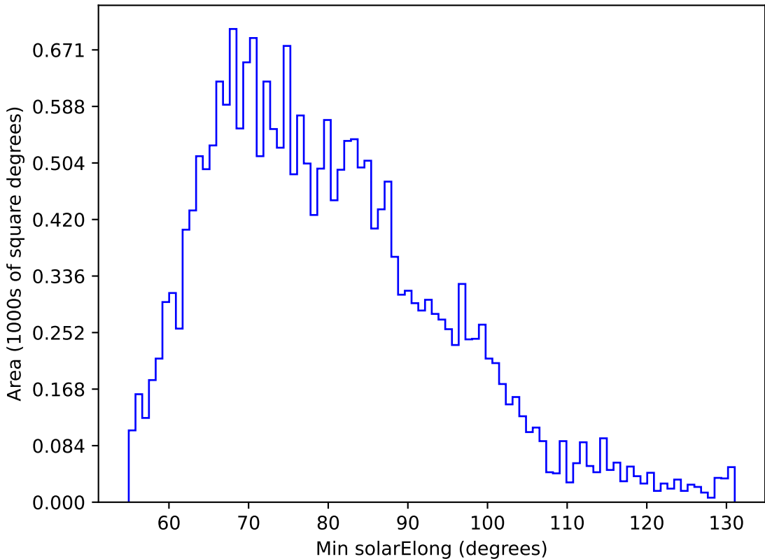
weather_cloudso12v3.4_10yrs All sky u band: Min solarElong
