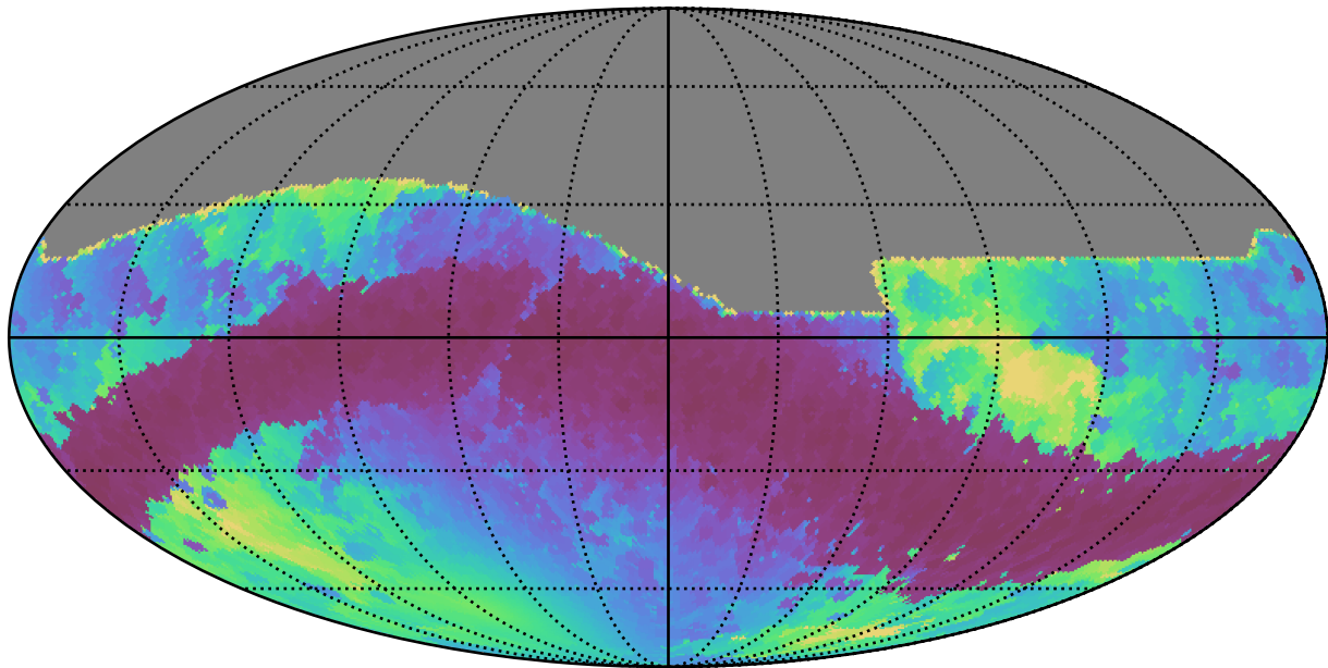
weather_cloudso12v3.4_10yrs All sky r band: Min solarElong
