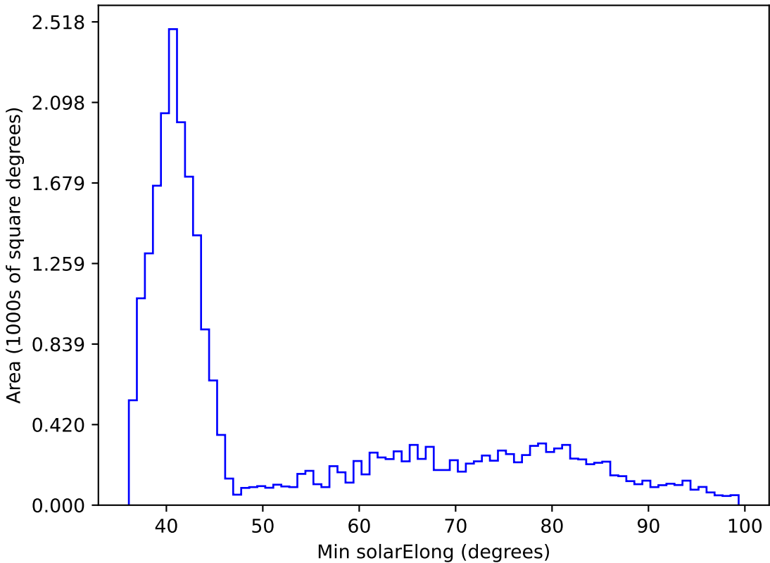
weather_cloudso12v3.4_10yrs All sky i band: Min solarElong
