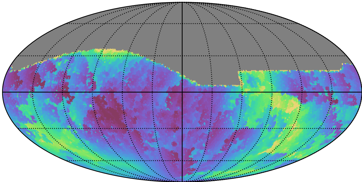
weather_cloudso12v3.4_10yrs All sky g band: Min solarElong
