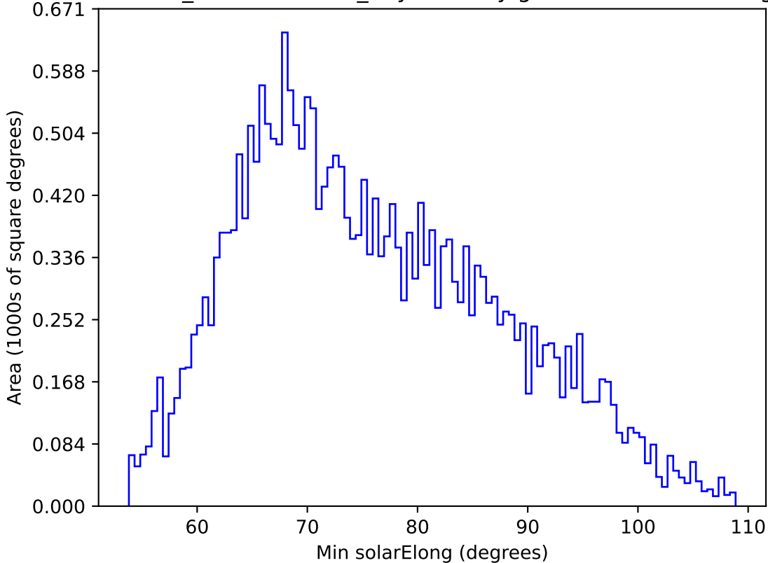
weather_cloudso12v3.4_10yrs All sky g band: Min solarElong
