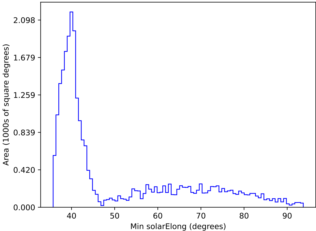
weather_cloudso12v3.4_10yrs All sky all bands: Min solarElong
