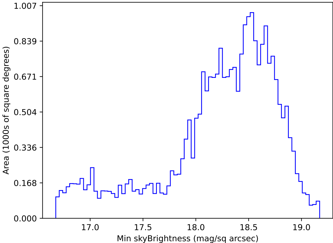
weather_cloudso12v3.4_10yrs Yr 1 z band: Min skyBrightness
