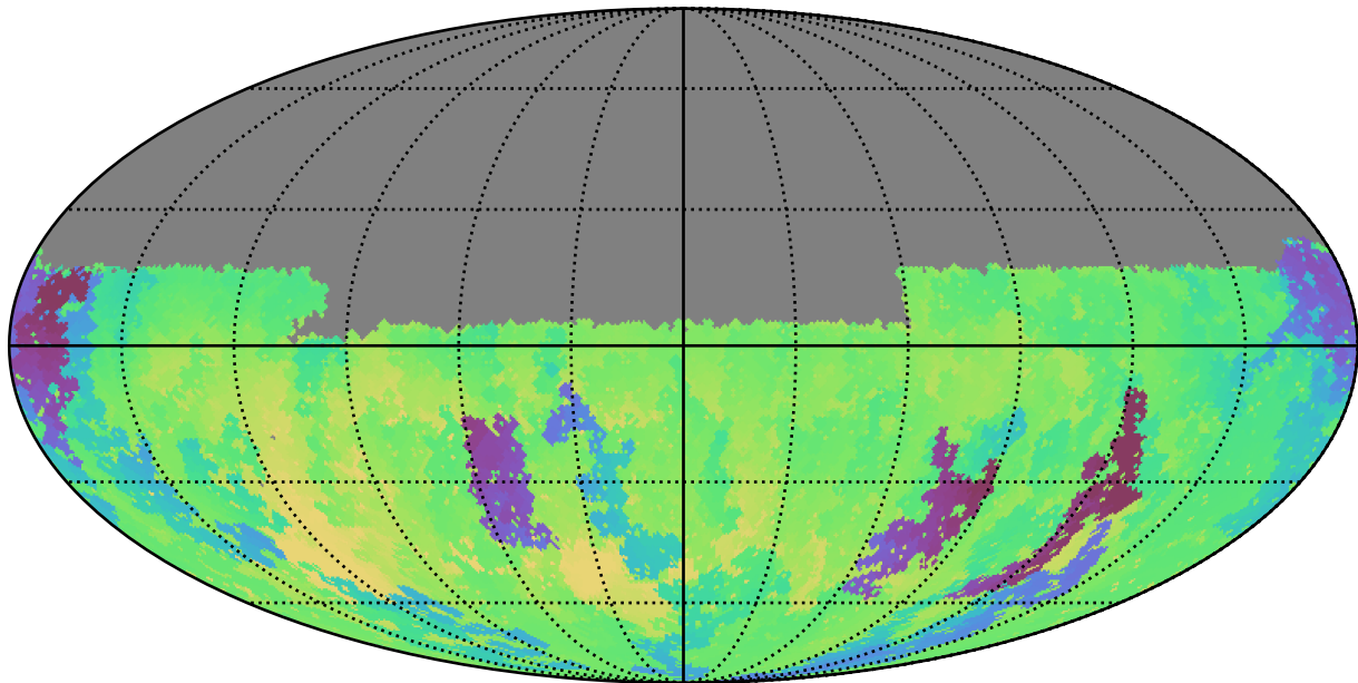
weather_cloudso12v3.4_10yrs Yr 1 u band: Min skyBrightness
