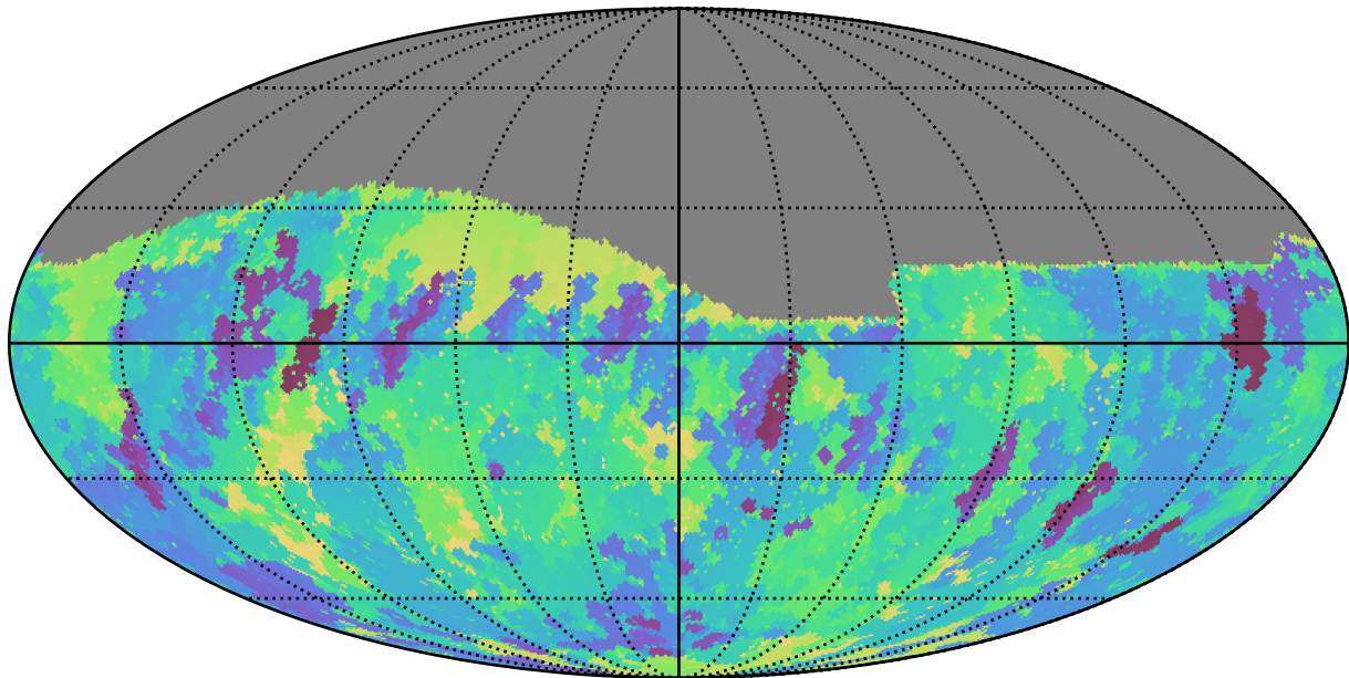
weather_cloudso12v3.4_10yrs Yr 1 r band: Min skyBrightness
