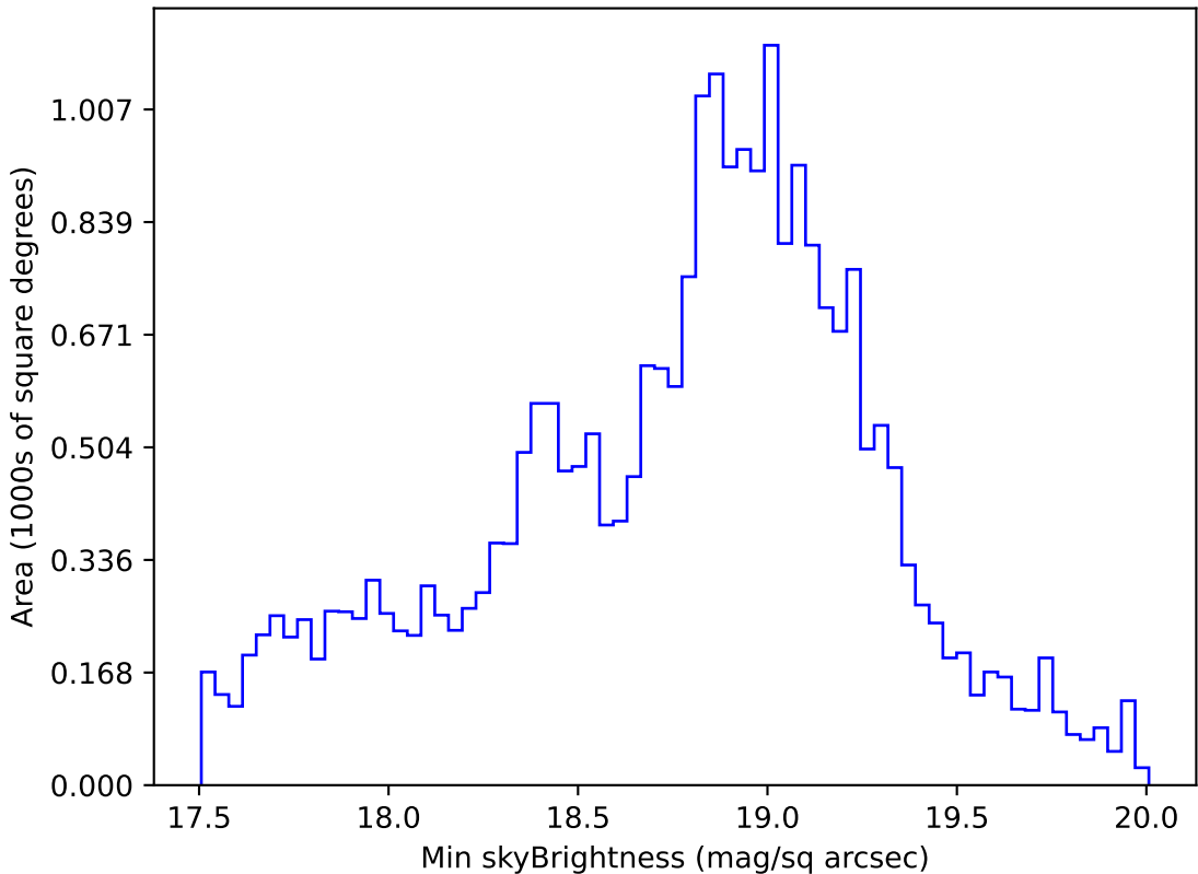
weather_cloudso12v3.4_10yrs Yr 1 i band: Min skyBrightness
