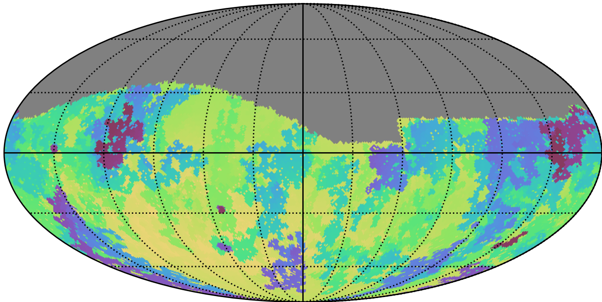
weather_cloudso12v3.4_10yrs Yr 1 g band: Min skyBrightness
