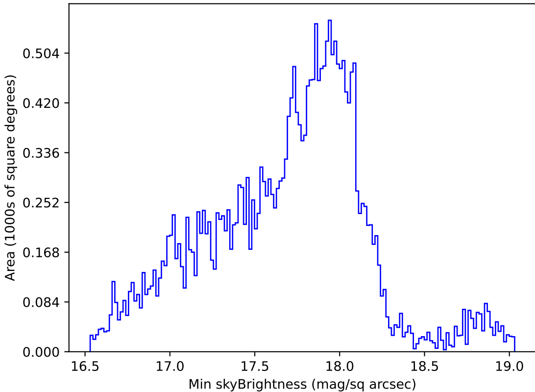
weather_cloudso12v3.4_10yrs Yr 1 all bands: Min skyBrightness
