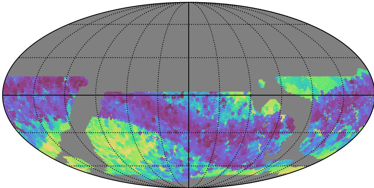
weather_cloudso12v3.4_10yrs WFD z band: Min skyBrightness
