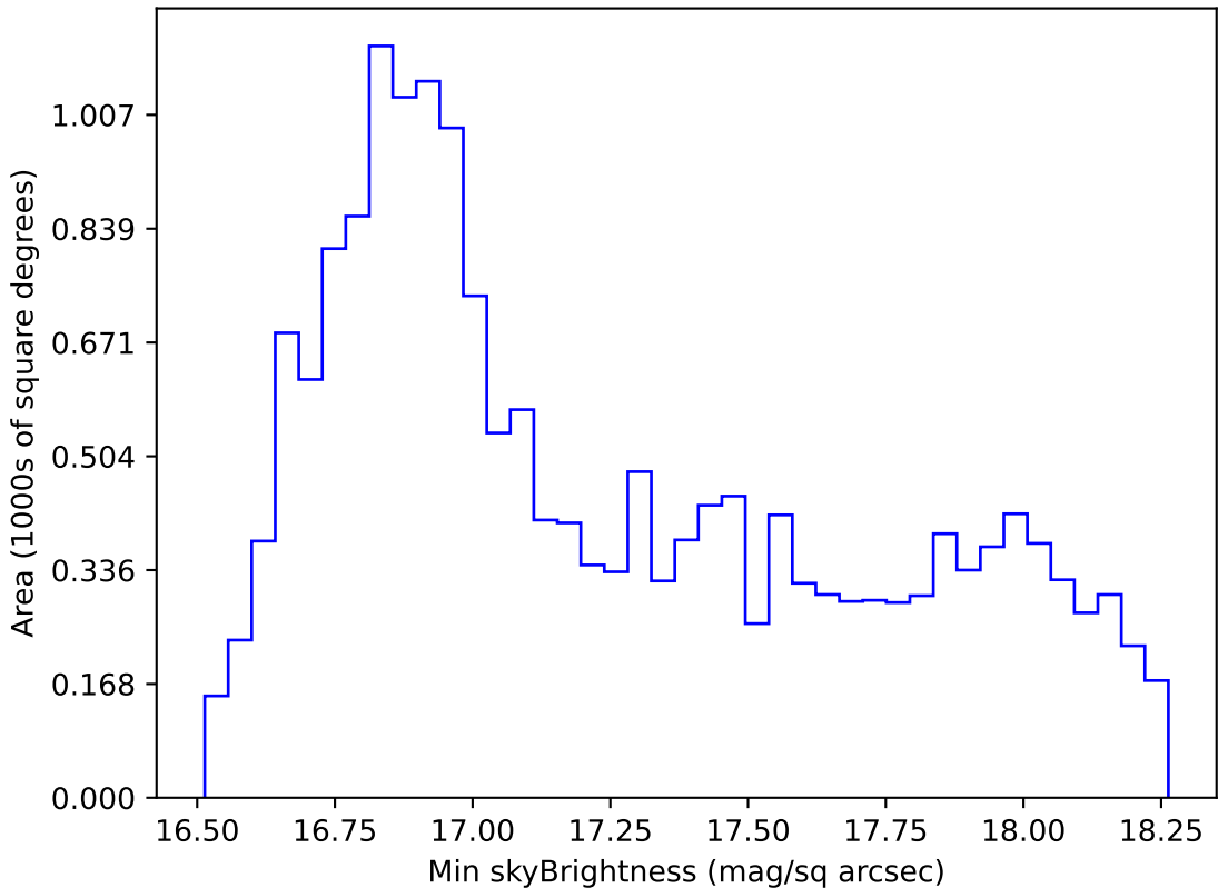
weather_cloudso12v3.4_10yrs WFD z band: Min skyBrightness
