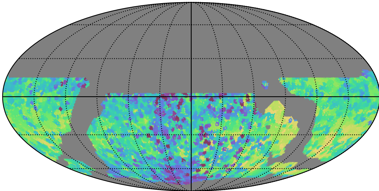
weather_cloudso12v3.4_10yrs WFD y band: Min skyBrightness
