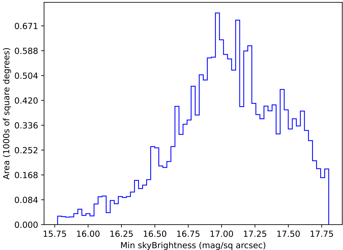
weather_cloudso12v3.4_10yrs WFD y band: Min skyBrightness
