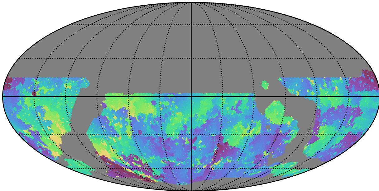
weather_cloudso12v3.4_10yrs WFD u band: Min skyBrightness
