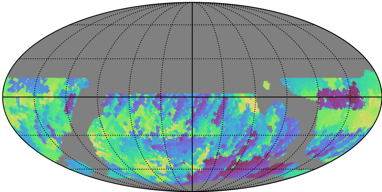
weather_cloudso12v3.4_10yrs WFD r band: Min skyBrightness
