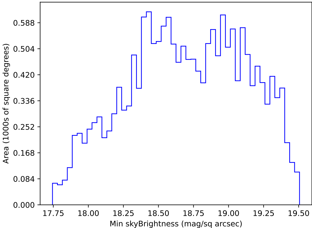
weather_cloudso12v3.4_10yrs WFD r band: Min skyBrightness
