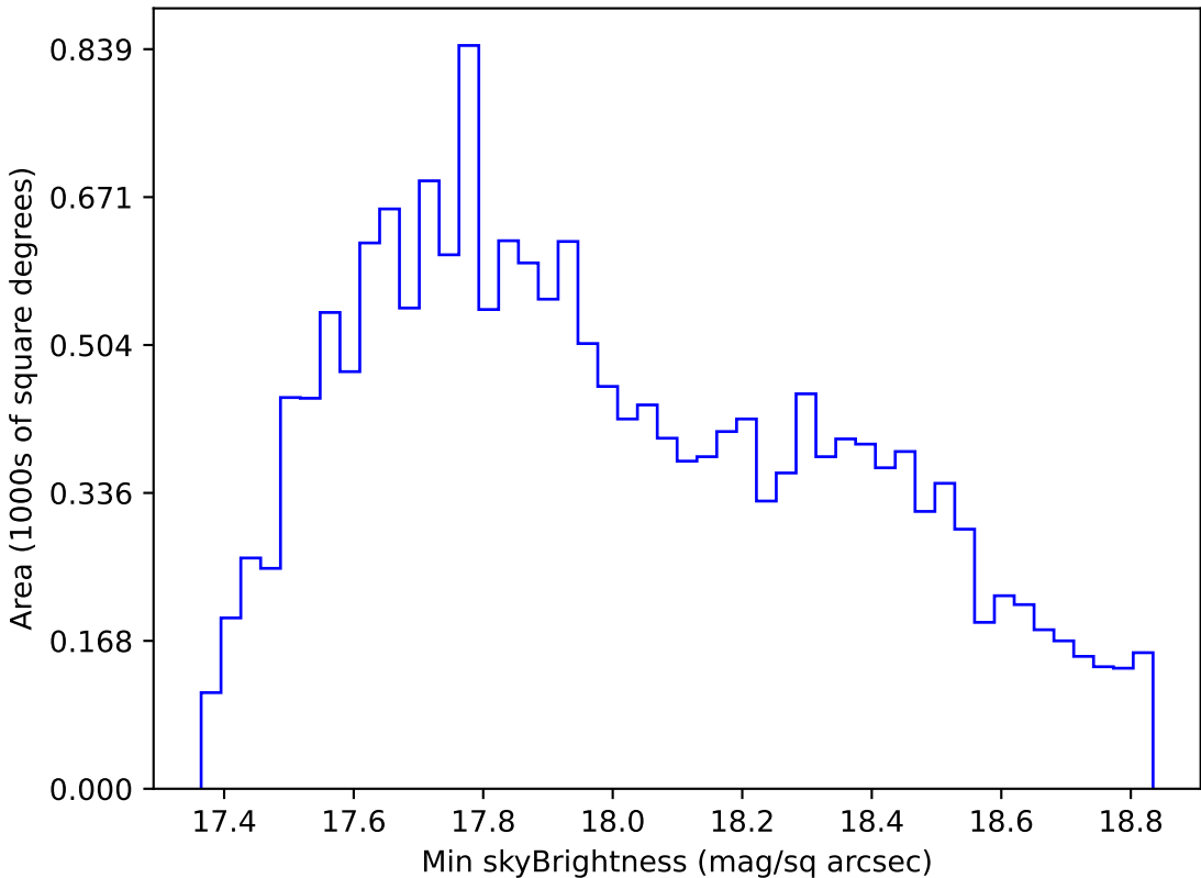
weather_cloudso12v3.4_10yrs WFD i band: Min skyBrightness
