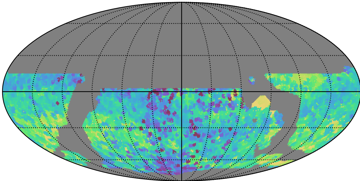
weather_cloudso12v3.4_10yrs WFD all bands: Min skyBrightness
