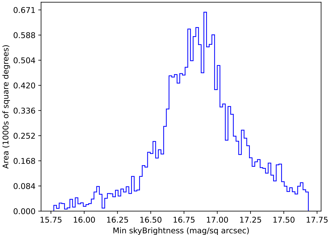
weather_cloudso12v3.4_10yrs WFD all bands: Min skyBrightness
