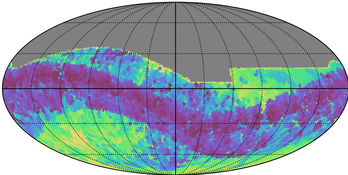
weather_cloudso12v3.4_10yrs All sky z band: Min skyBrightness
