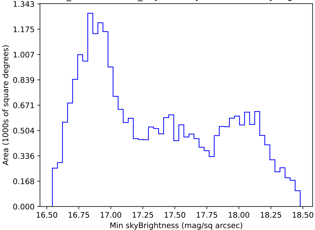
weather_cloudso12v3.4_10yrs All sky z band: Min skyBrightness
